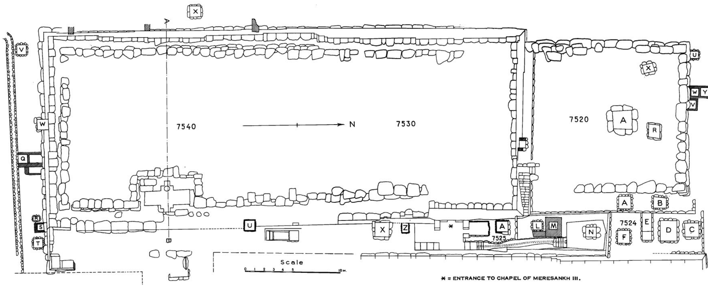
Plan B. Plan of G 7520-7540.
