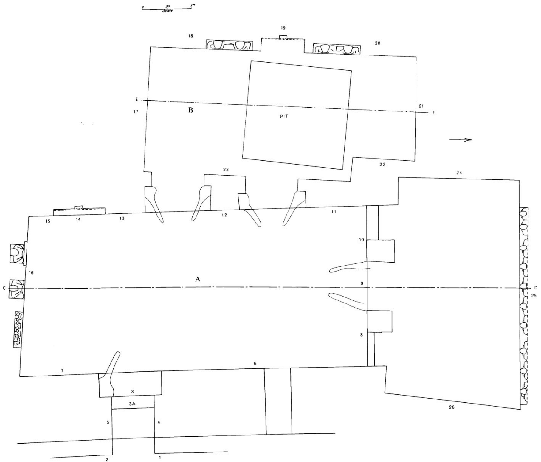
Plan C. Plan of Chambers, G 7530 sub.
